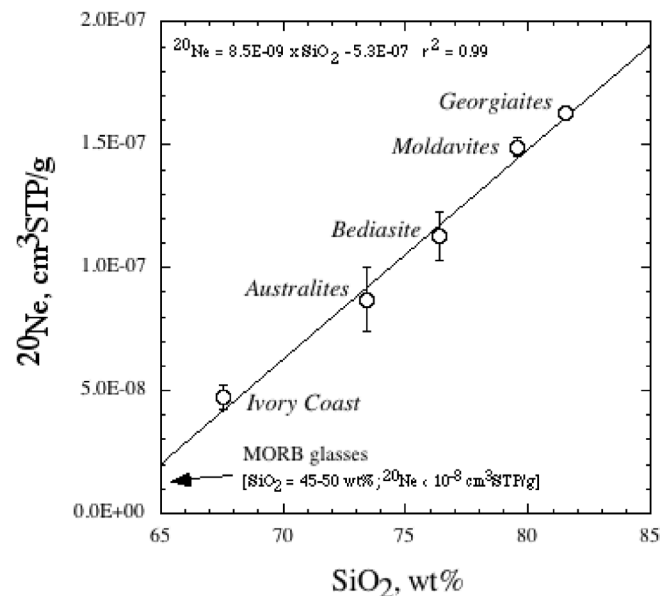
Fig. 5. Average ^{20}\text{Ne} concentration in splash-form tektites calculated for each strewn field plotted against the average \text{SiO}_2 content. See the text for data sources. The arrow indicates the ^{20}\text{Ne} concentrations and \text{SiO}_2 contents characteristics of MORB glasses (internal compilation of literature data).
