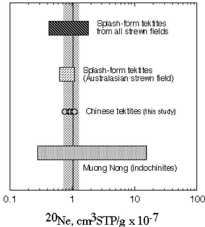
Fig. 4. Range of ^{20}\text{Ne} concentration in splash-form tektites (Hennecke et al. 1975; Matsubara and Matsuda 1991; Matsuda et al. 1993, 1996; Palma et al. 1997), Muong Nong tektites (Murty 1997; Mizote et al. 2003), and Chinese tektites (this study). The dashed line and dotted area represent the average ^{20}\text{Ne} concentration in splash-form tektites and its standard deviation, respectively. Note that the x-axis is in log scale.
